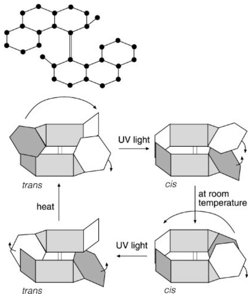
30. A scratch-built molecular rotary motor powered by light. The top image shows the carbon-atom framework.
