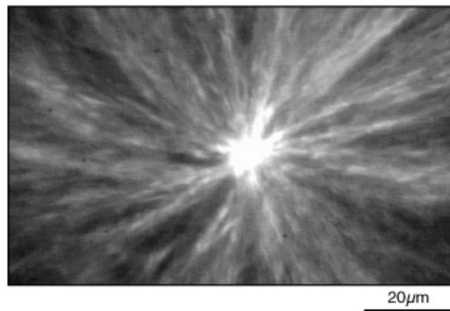
31. Microtubules organized into star-shaped structures by semi-synthetic molecular motors made from modified proteins.
