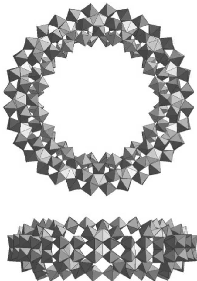
10. A molecular ‘big wheel’ made by Achim Müller’s group in Germany (top and side views). Each pyramid is a cluster of molybdenum and oxygen atoms.
