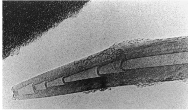
20. The tapering tip of a carbon nanotube, seen in cross-section in the electron microscope.
